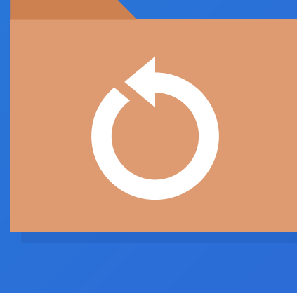
Restoring backups
